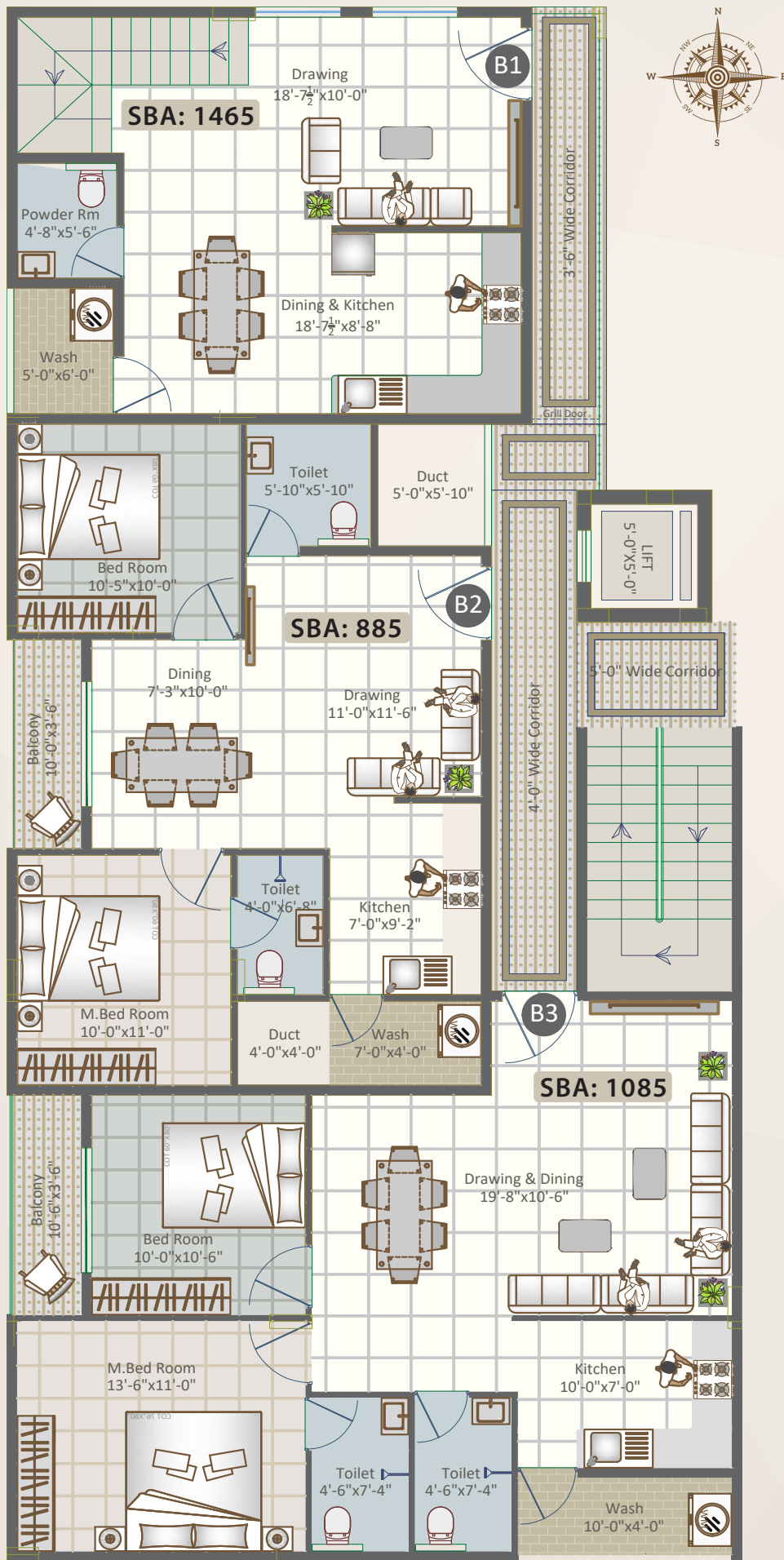
Ground & Second Floor Master Plan
